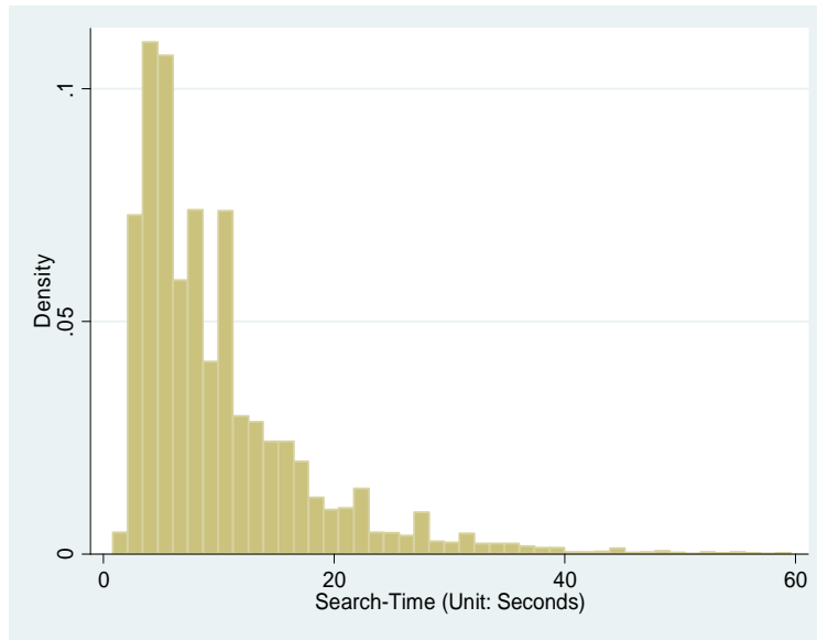
Figure 2: Search-Time Histogram
